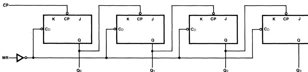
LOGIC DIAGRAM (one half shown)
