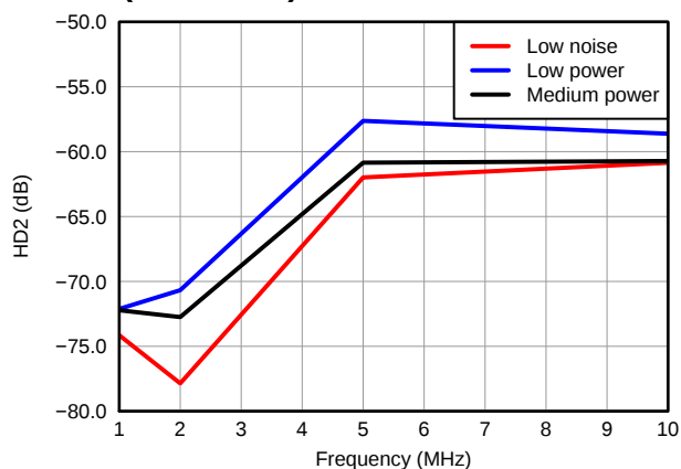
Figure 37. HD2 vs. Frequency, V_{in} = 500 \text{ mV}_{PP} and V_{OUT} = -1 \text{ dBFS}
