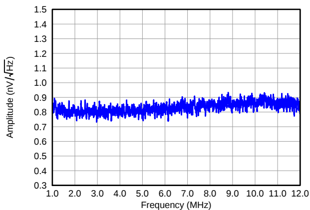
Figure 27. IRN, PGA = 24 dB and Low Noise Mode
