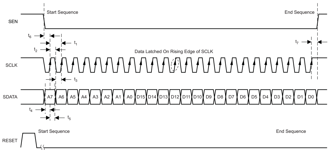
Figure 60. SPI Timing
