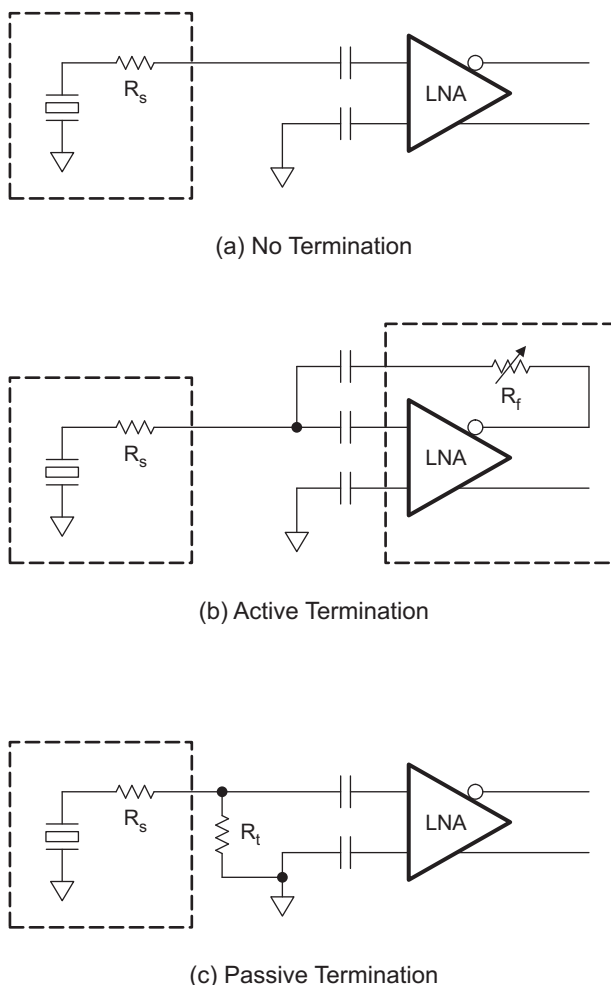
Figure 84. Termination Configurations
