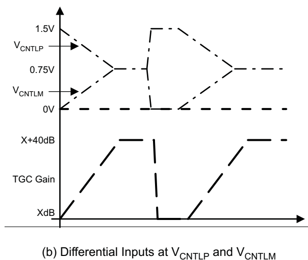
Figure 86. V_{\text{CNTLP}} and V_{\text{CNTLM}} Configurations
